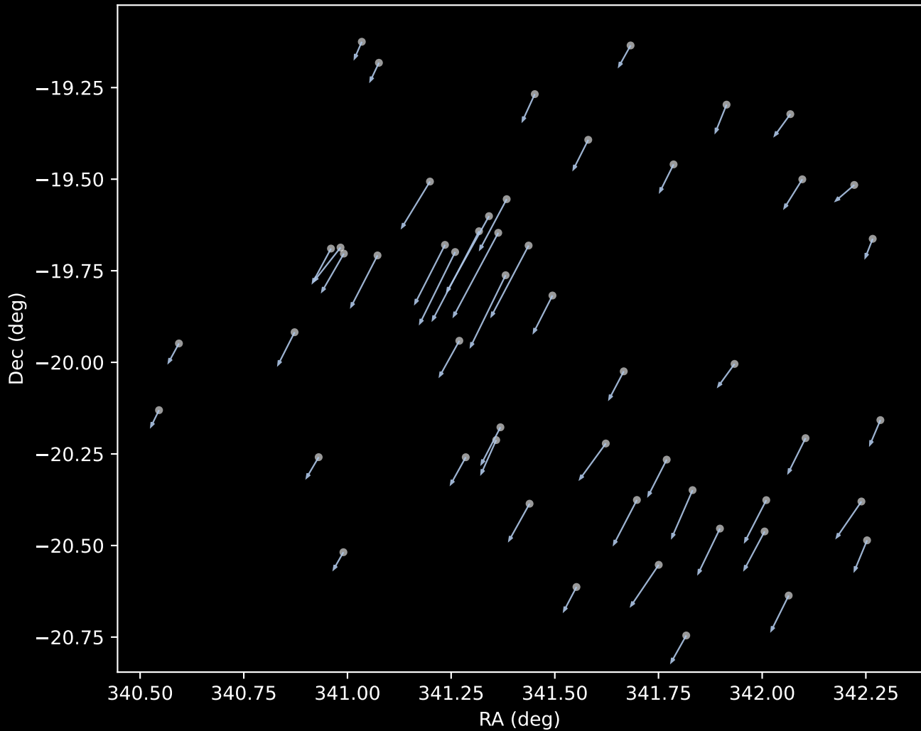
APOGEE DR17 Cluster 1 Proper Motion Vectors (n=52)
