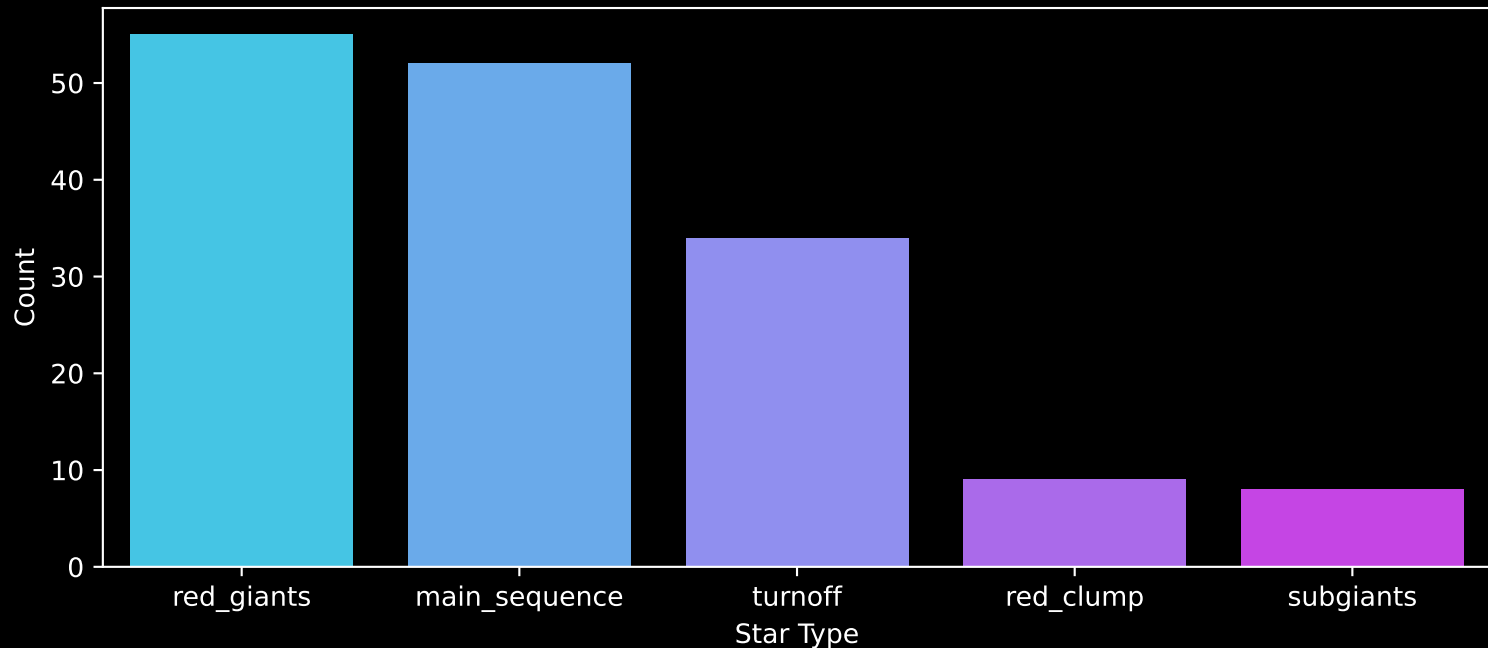
APOGEE DR17 Field: [353+24-O] Count plot of Star Type
