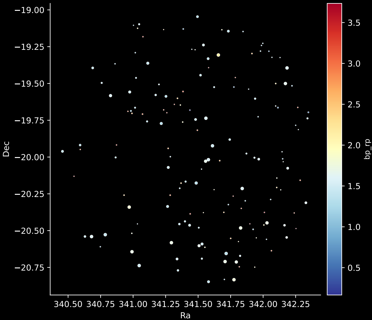
APOGEE DR17 Field: [353+24-O] Stars: 158
