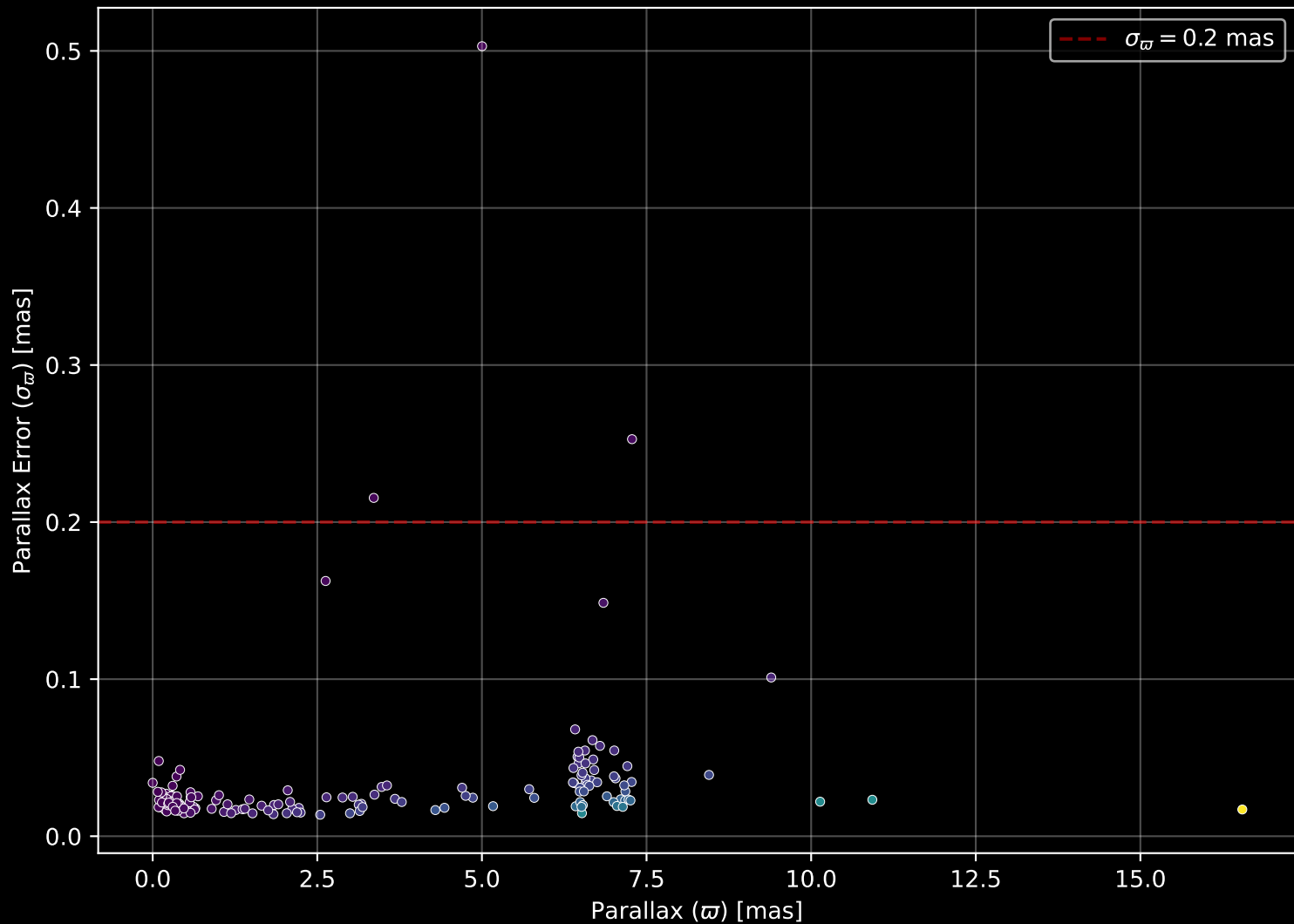
APOGEE DR17 Field: [353+24-O] Parallax Quality (n= 158)
