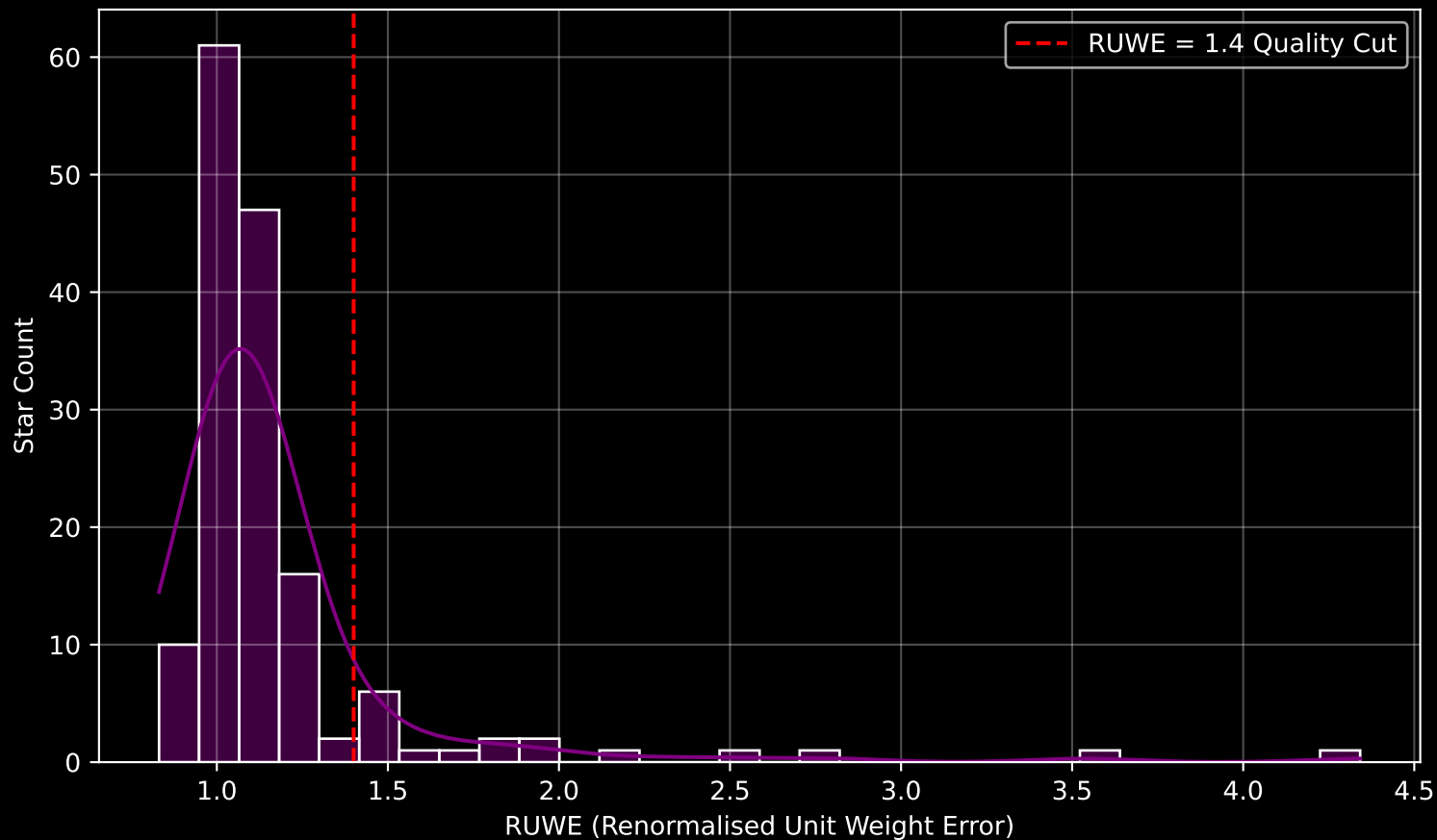
GAPOGEE DR17 Field [353+24-O] RUWE Distribution (n= 153)
