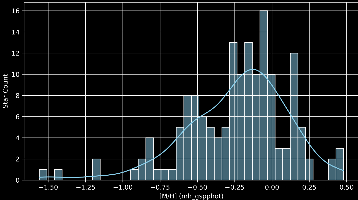
APOGEE DR17 Field: [353+24-O [M/H] (mh_gspphot) (n= 157)
