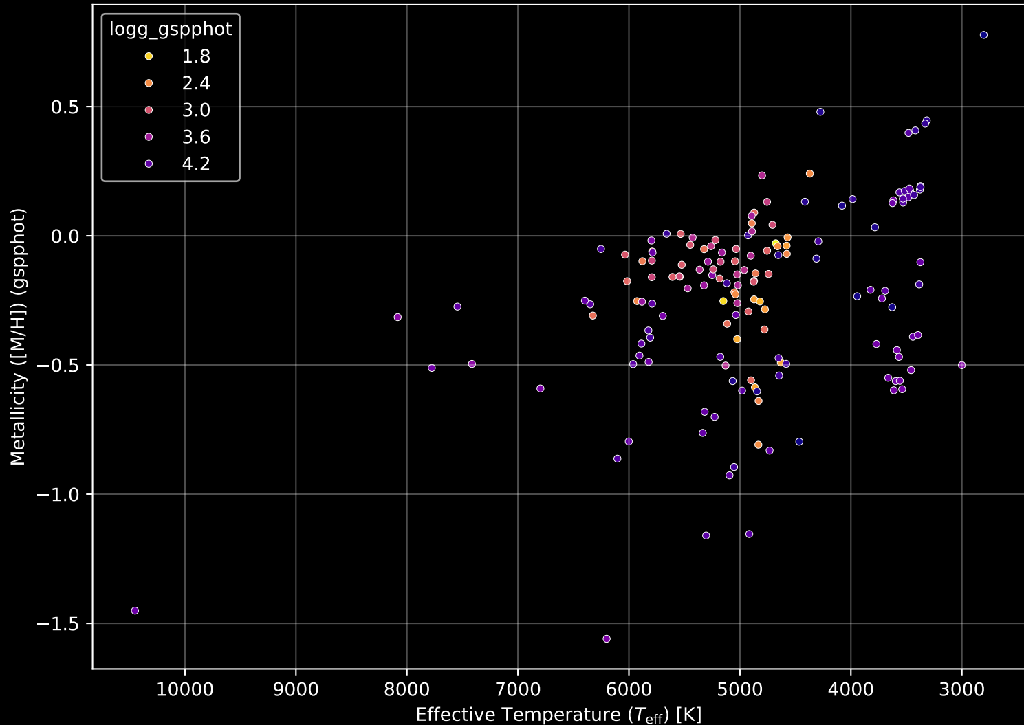
APOGEE DR17 Field: [353+24-O] Stellar Population Parameters (n= 158)
