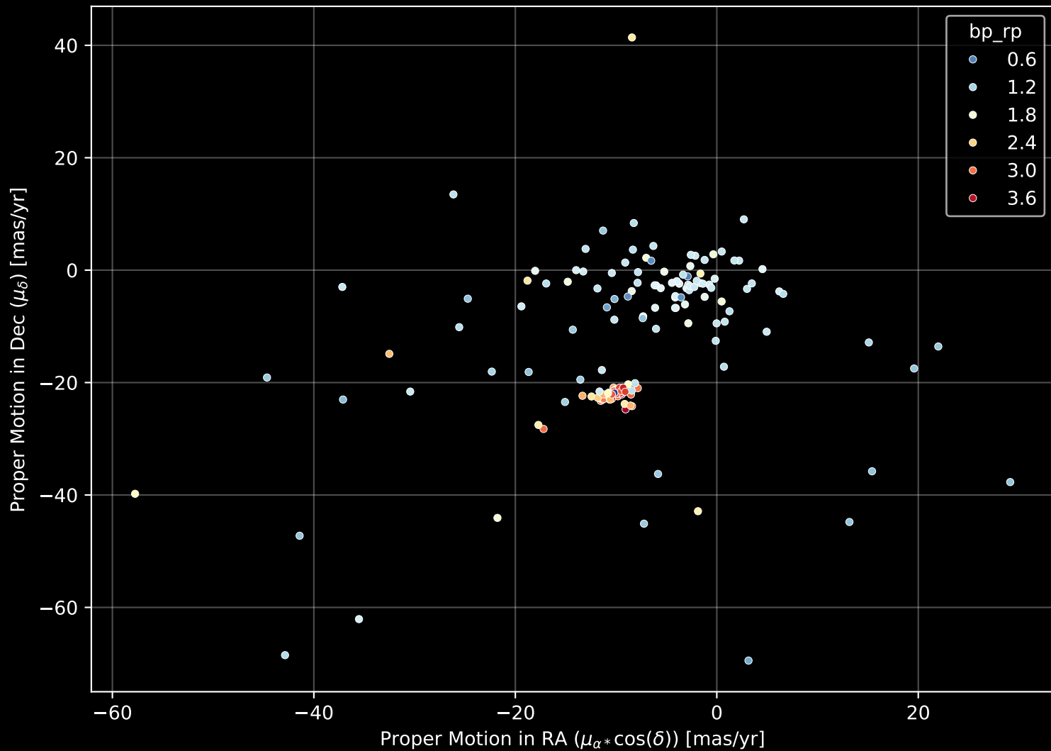
APOGEE DR17 Field: [353+24-O] Proper Motion Diagram (n= 158)
